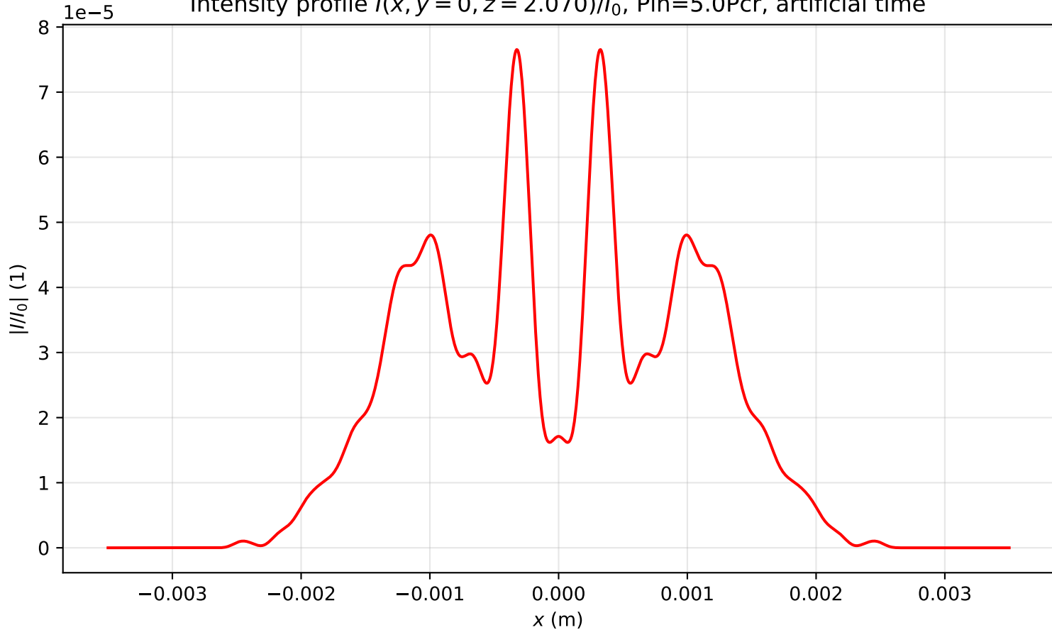
Intensity profile I(x, y = 0, z = 2.070)/I_0 , P_{in}=5.0P_{cr} , artificial time
